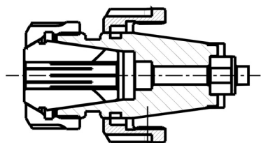
Adapter UNI CHANGE with pliers ER
