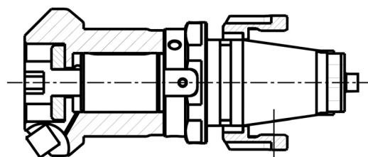
Adapter UNI CHANGE with pliers ER
