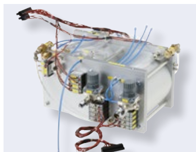
Gas mixing unit for medical use
