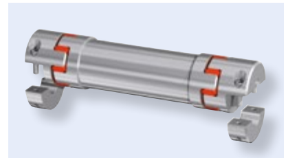
Line Shaft
